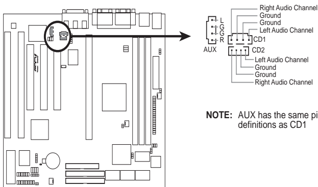
P2L-VM/P2E-VM Stereo Audio In Connectors
